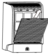
3. Lift up to remove the back panel
